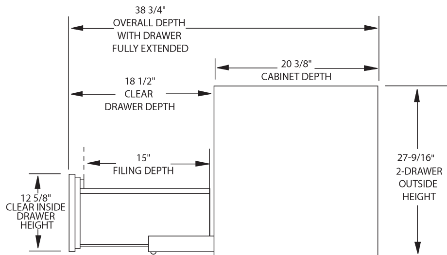
SIDE VIEW
